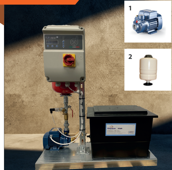
1. Pedrollo PKm 60 Pump (Stock Code: 1000009) 2. 8L Global Sphere Pressure Vessel (Stock Code: 1004918)
